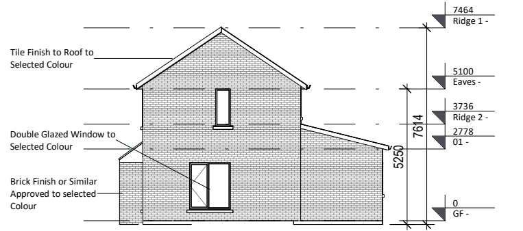
⑧ Side Elevation End of Terrace with Gable Windows Full Brick 1 : 200
