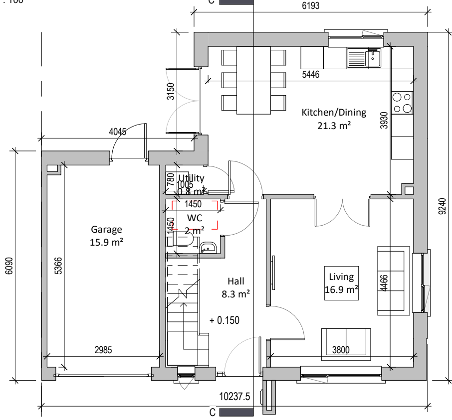
① Ground Floor End of Terrace with Gable Window 1 : 100
