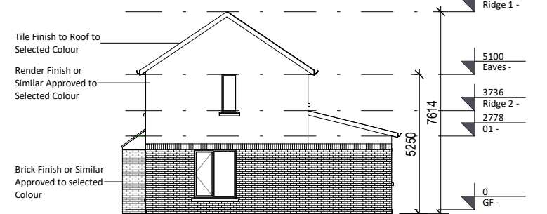
⑤ Side Elevation End Terrace with Gable Windows 1 : 200
