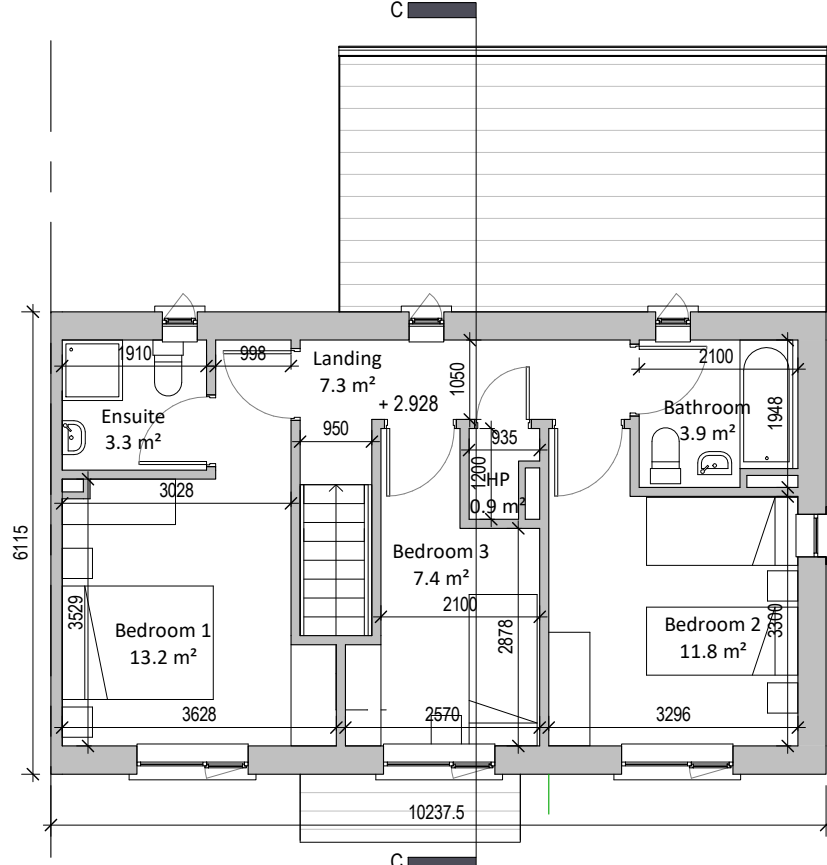
② First Floor End of Terrace with Gable Window 1 : 100
